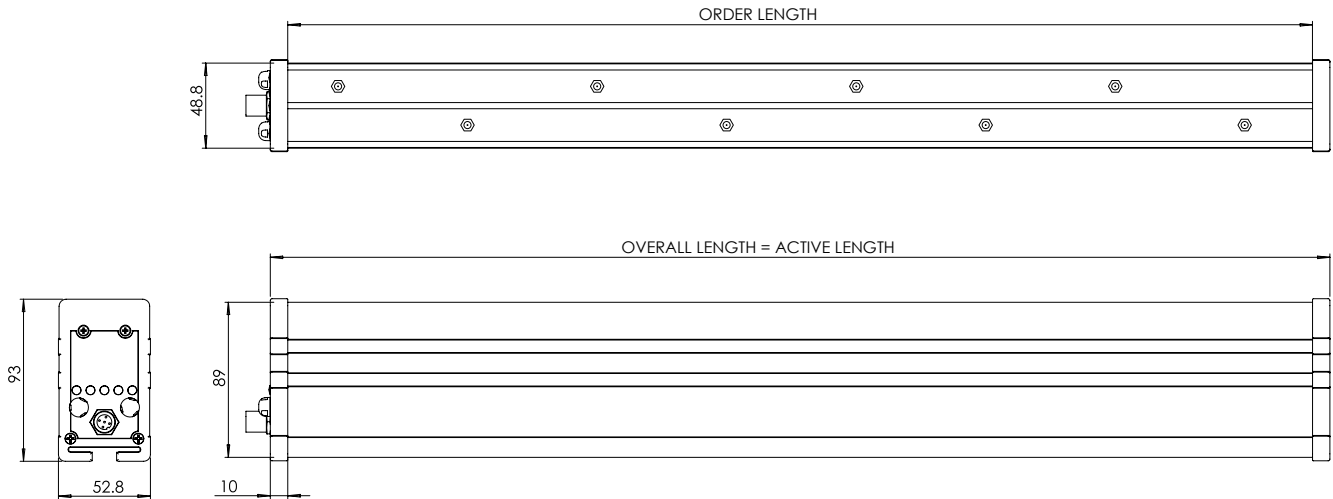
ALL DIMENSIONS IN MILLIMETRES
