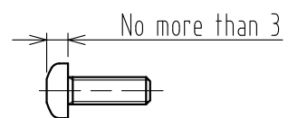
Screw Dimensions
